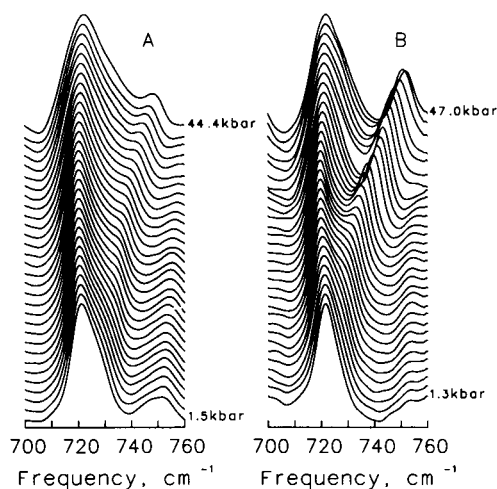
FIGURE 5 Comparison of the stacked contour plots of the infrared spectra in the \nu\text{CH}_2 region between the crystalline DMPC (A) and the aqueous DMPC bilayers (B).
