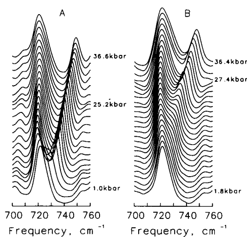
FIGURE 6 Comparison of the stacked contour plots of the infrared spectra in the \nu\text{CH}_2 region between the interdigitated DMPC bilayers (A) and the aqueous DMPC bilayers (B).
